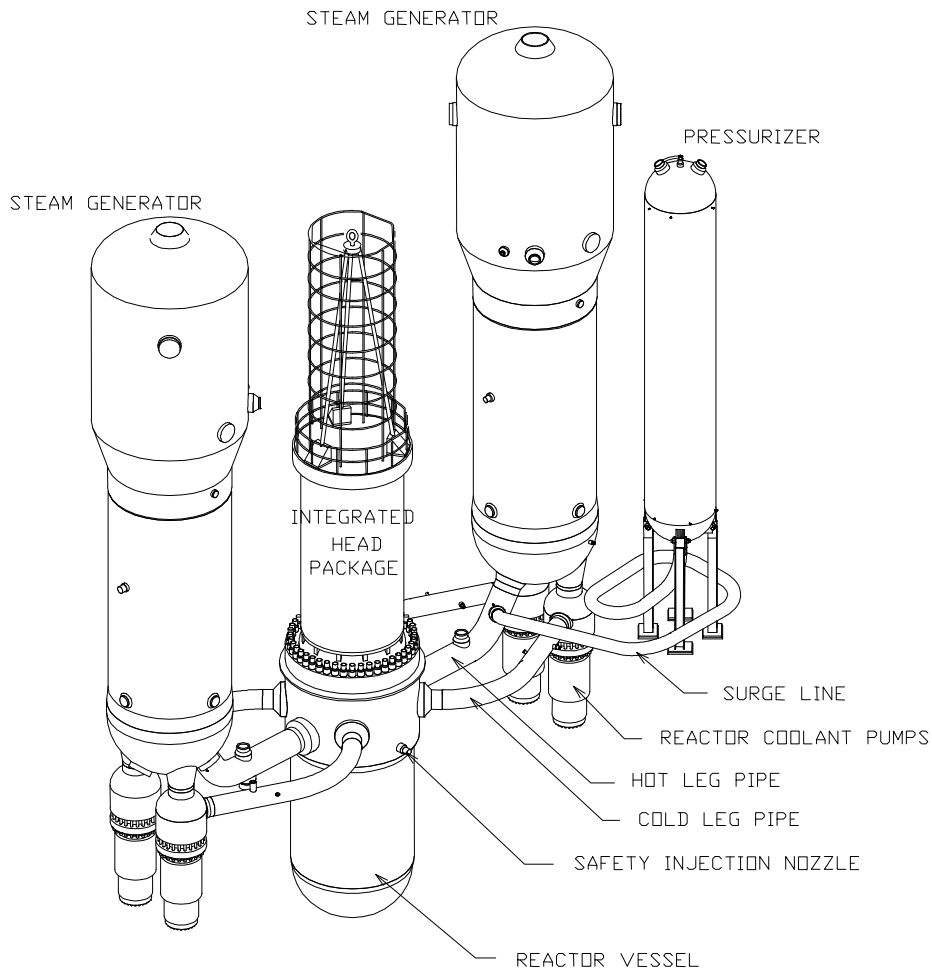
Figure 3 – AP1000 Reactor Coolant System
