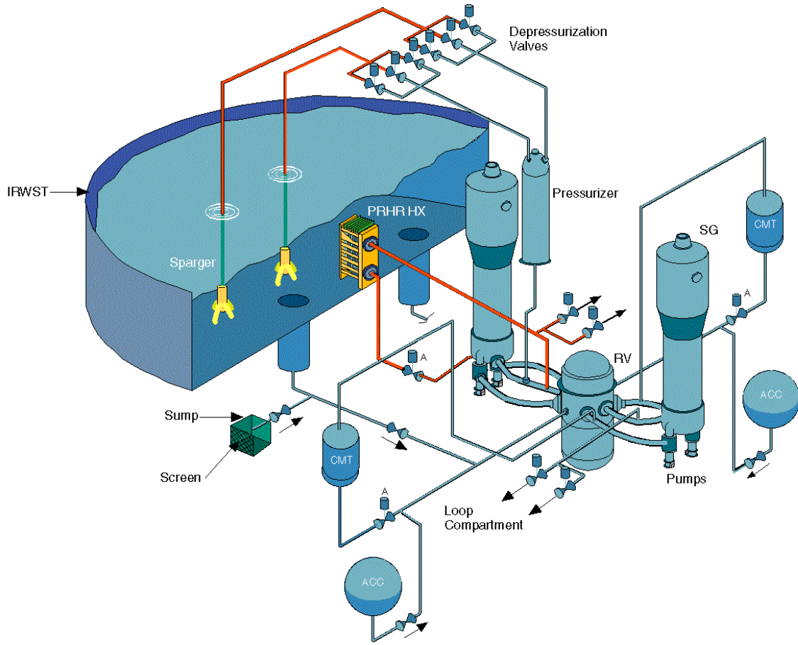
Figure 4 – AP1000 RCS and Passive Core Cooling System
